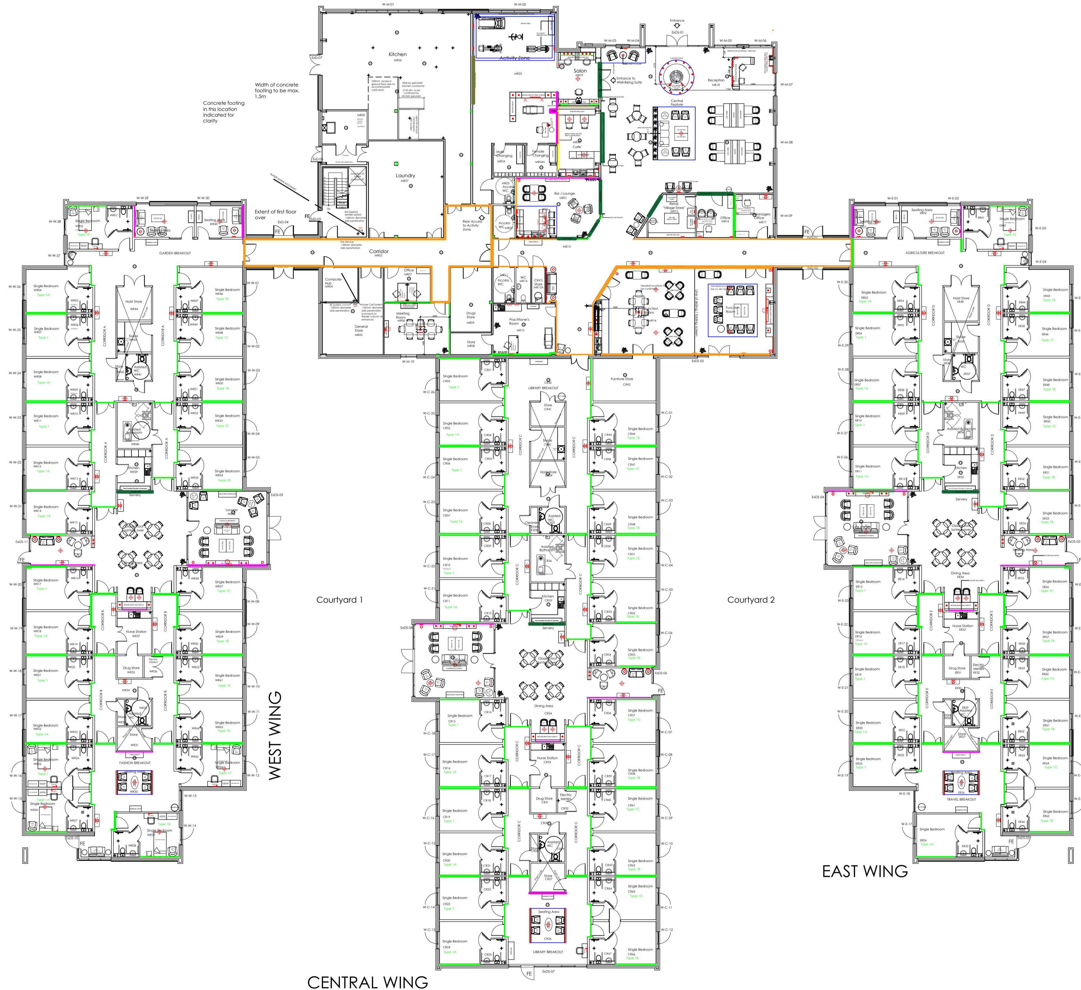
GROUND FLOOR COORDINATION PLAN
